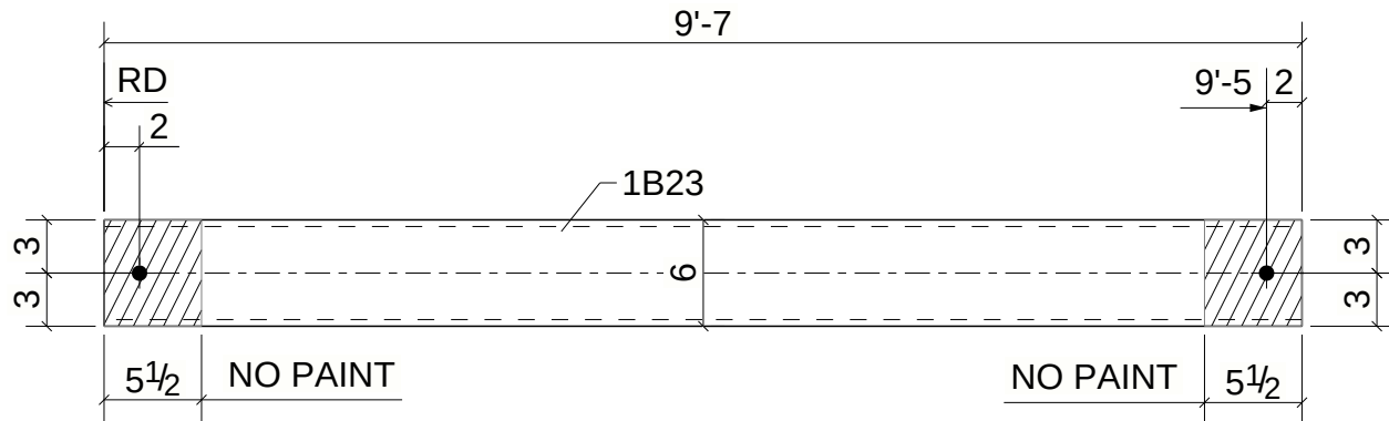
2 - HSS GIRTS - 1B23
